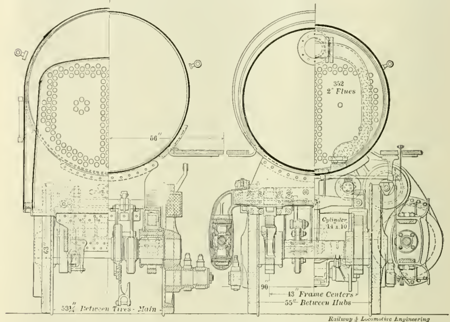
CROSS SECTIONS OF BROOKS TANDEM.
